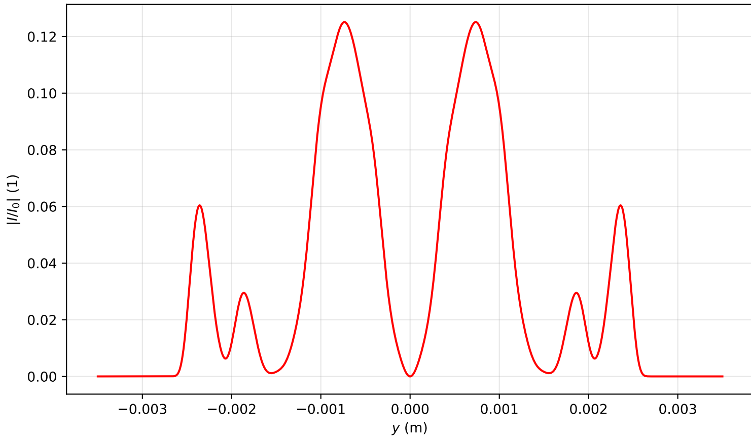
Intensity profile I(x=0, y, z=3.901)/I_0 , \text{Pin}=9.0\text{Pcr} , artificial time
